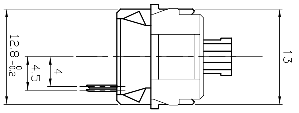
下視圖 CONNECTIONS (BOTTOM VIEW)
