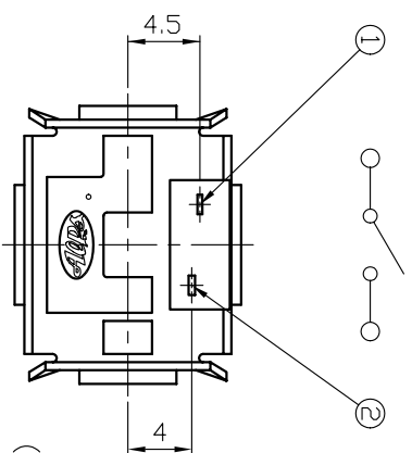
下視圖 CONNECTIONS (BOTTOM VIEW)
